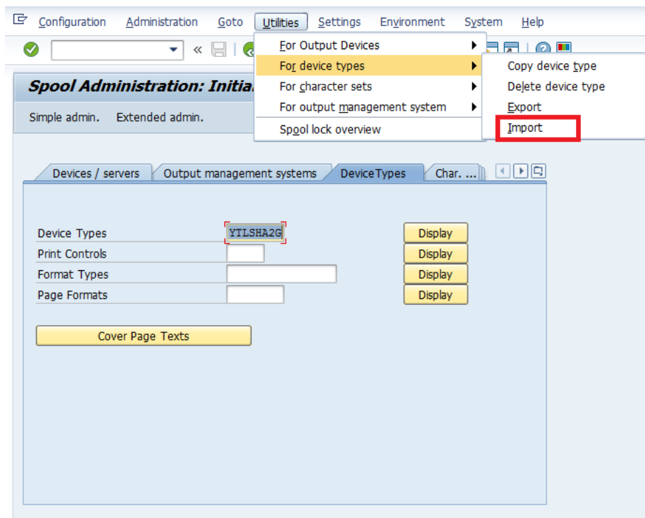
Figure 14: Importing Device Type file-1
