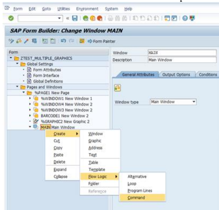
Figure 42 : Creating Command Node in Smart form by right clicking the Main Window.
