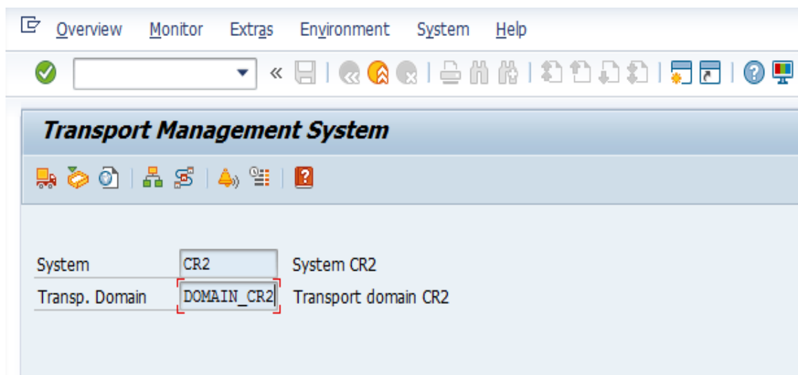
Figure 5 : Transaction STMS
