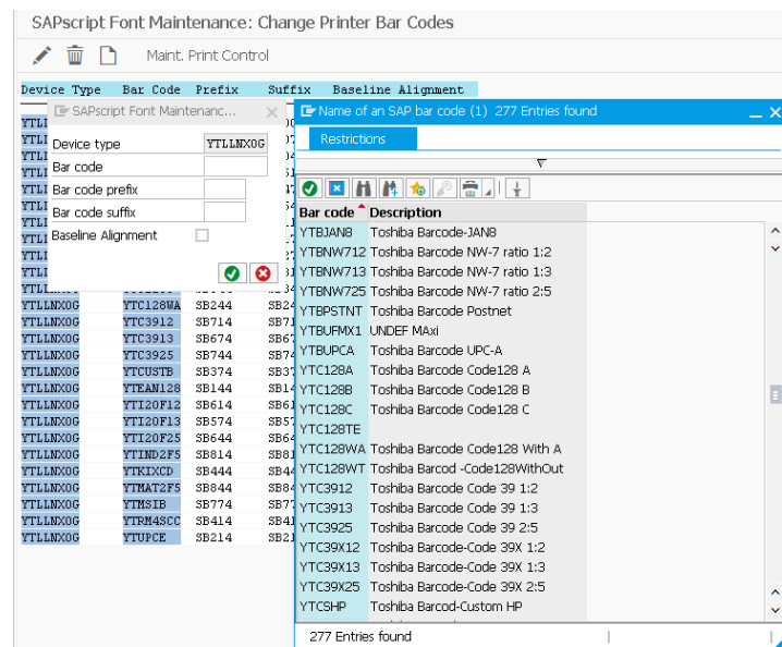
Figure 40 : Selecting System Bar code from entry list
