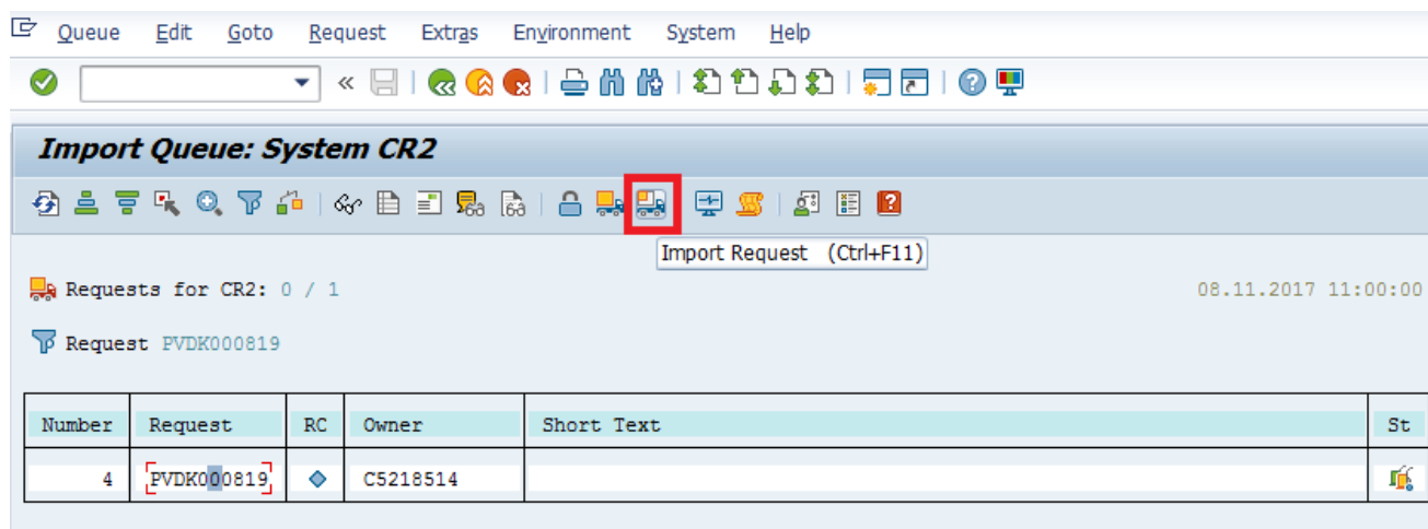
Figure 12 : Import Request
